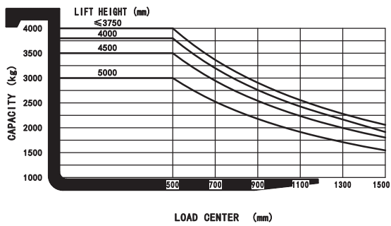
CAPACITY CHART
